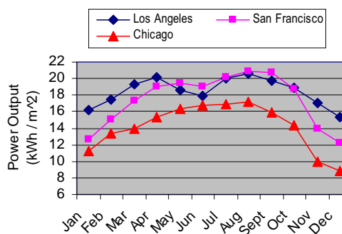
Figure 2: 35 deg. Tilt BIPV Power Output
