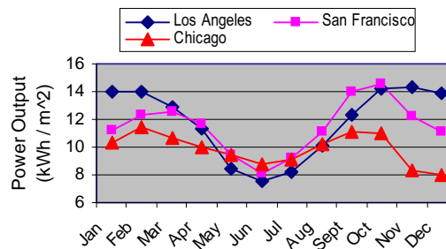
Figure 1: Vertical BIPV Power Output
